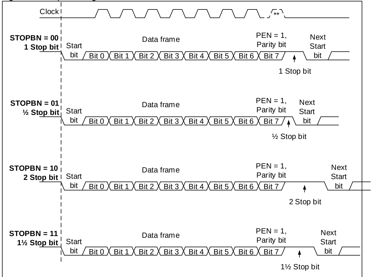
Figure 12-4 Stop bit configuration
