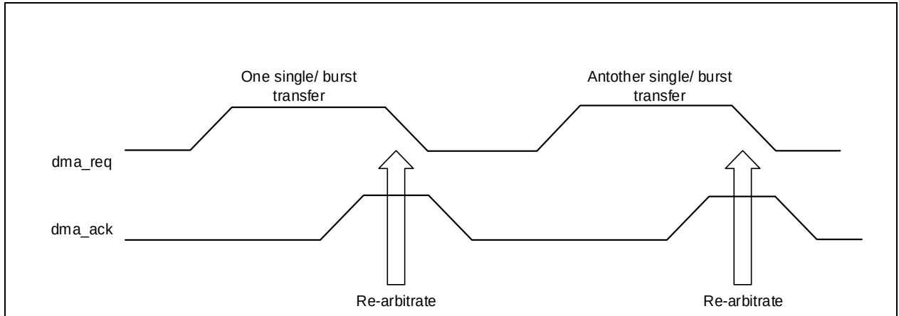
Figure 29-3 Re-arbitrae after Request/Acknowledge
