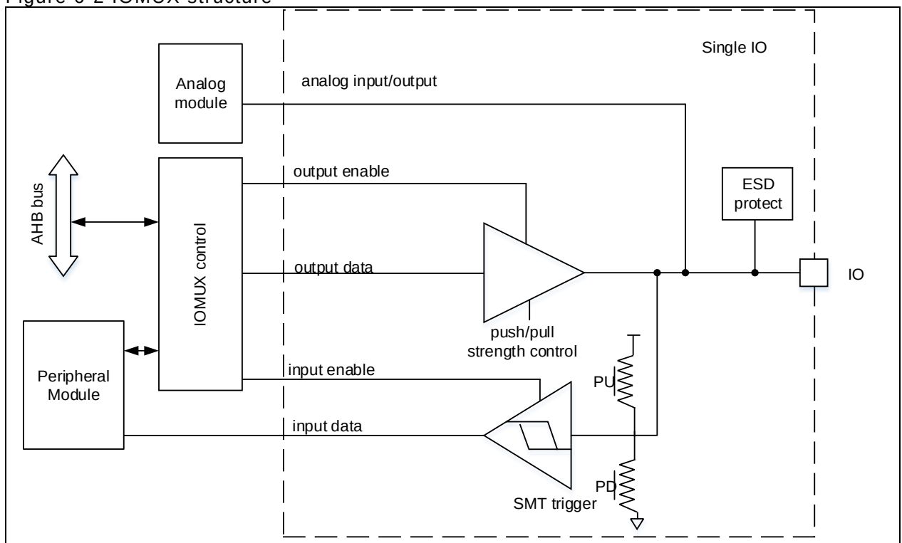
Figure 6-2 IOMUX structure
