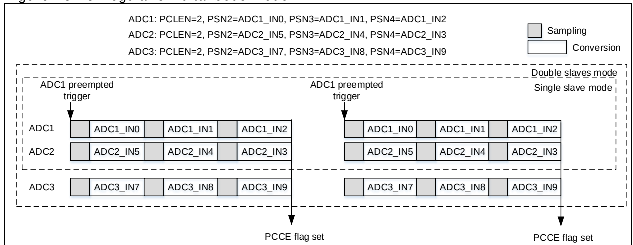
Figure 18-15 Regular simultaneous mode
