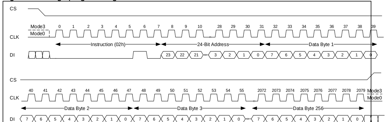
Figure 28-4 Page programming
