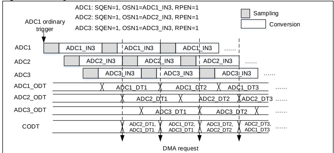
Figure 18-18 Regular shift mode and DMA mode 2
