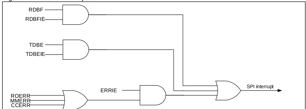
Figure 13-15 SPI interrupts
