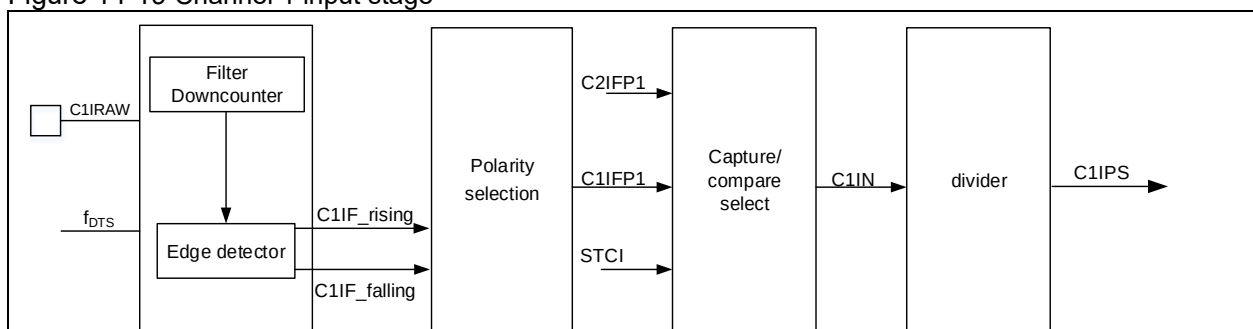
Figure 14-19 Channel 1 input stage
