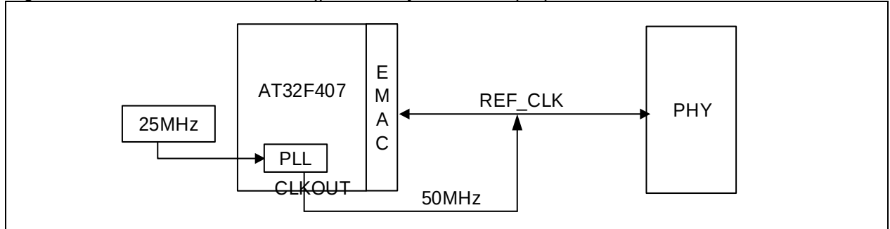
Figure 26-8 RMII clock sources (provide by an external crystal oscillator)
