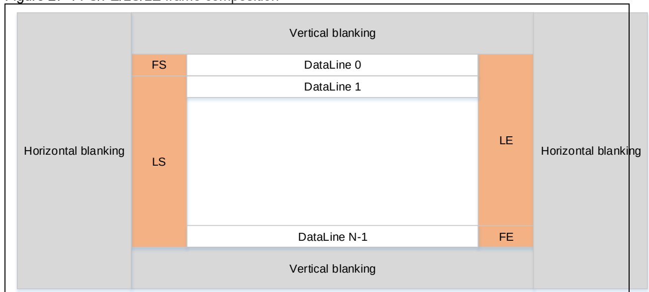
Figure 27-4 FS/FE/LS/LE frame composition
