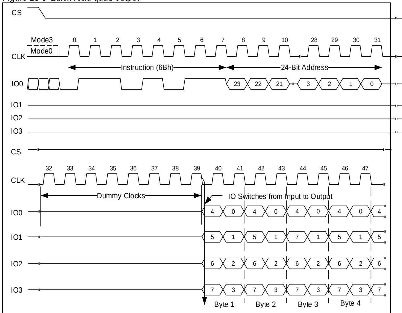
Figure 28-9 Quick read quad output
