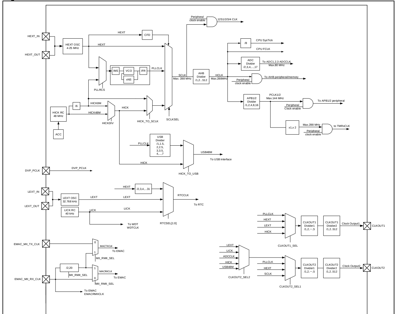
Figure 4-1 AT32F435/437 clock tree
