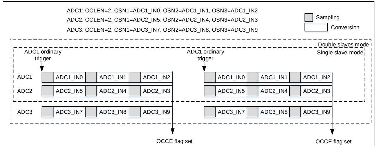
Figure 18-14 Regular simultaneous mode
