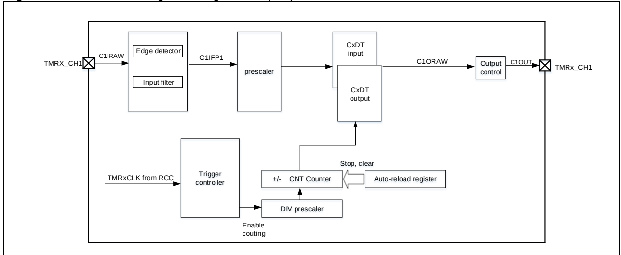
Figure 14-33 Block diagram of general-purpose TMR10/11/13/14
