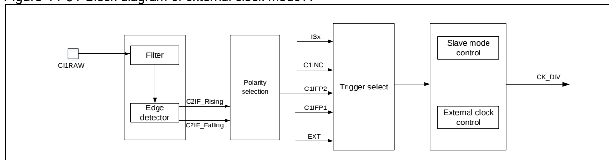
Figure 14-51 Block diagram of external clock mode A
