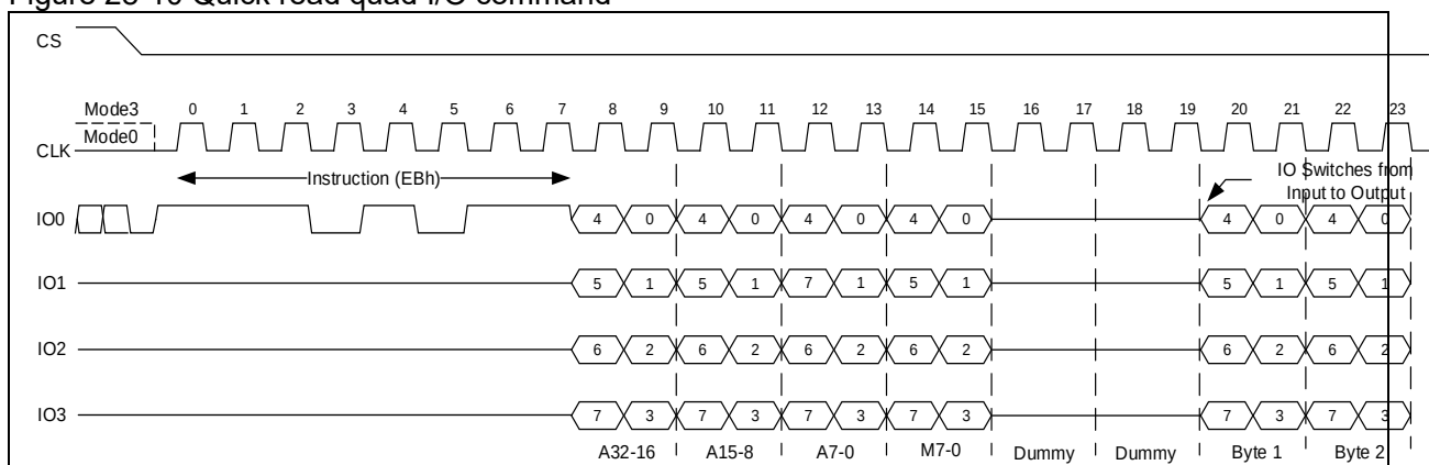
Figure 28-10 Quick read quad I/O command
