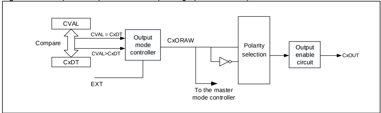
Figure 14-20 Capture/compare channel output stage (channel 1 to 4)
