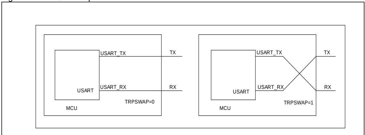
Figure 12-7 Tx/Rx swap
