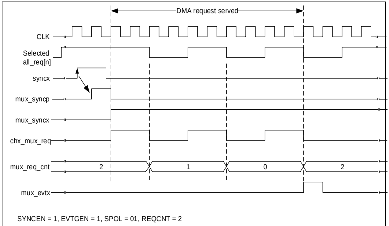
Figure 29-13 DMAMUX event generation
