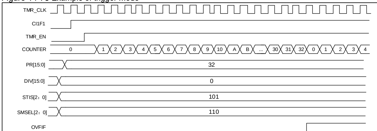
Figure 14-75 Example of trigger mode
