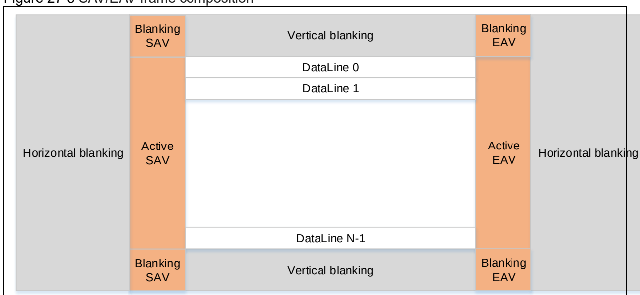
Figure 27-5 SAV/EAV frame composition
