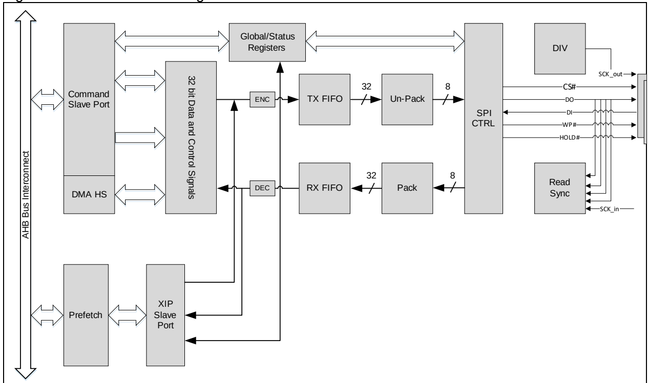
Figure 28-1 Function block diagram
