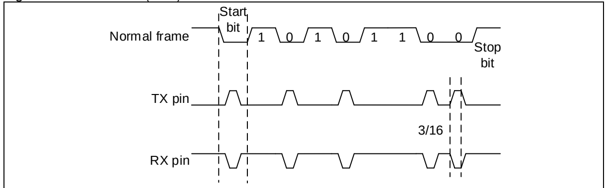
Figure 12-2 IrDA DATA(3/16) – normal mode
