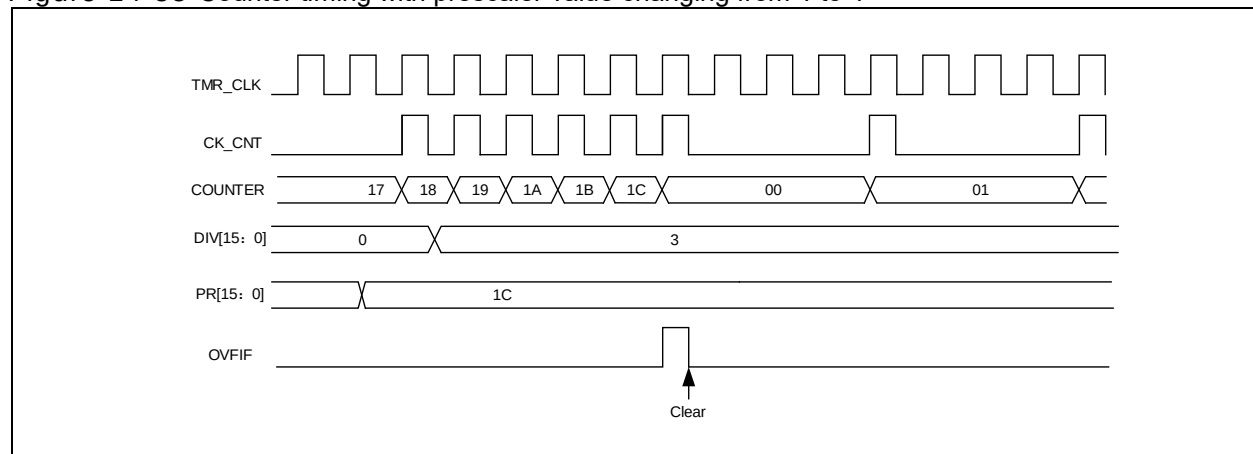
Figure 14-55 Counter timing with prescaler value changing from 1 to 4
