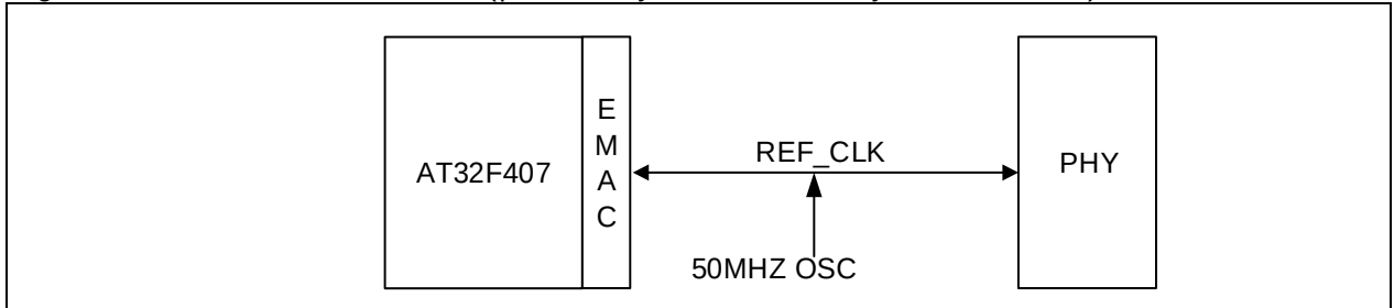
Figure 26-8 RMII clock sources (provide by an external crystal oscillator)
