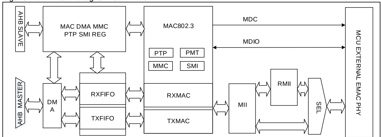
Figure 26-1 Block diagram of EMAC
