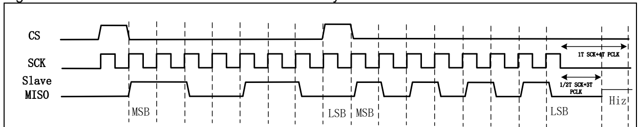
Figure 13-14 TI mode continous transfer with dummy CLK
