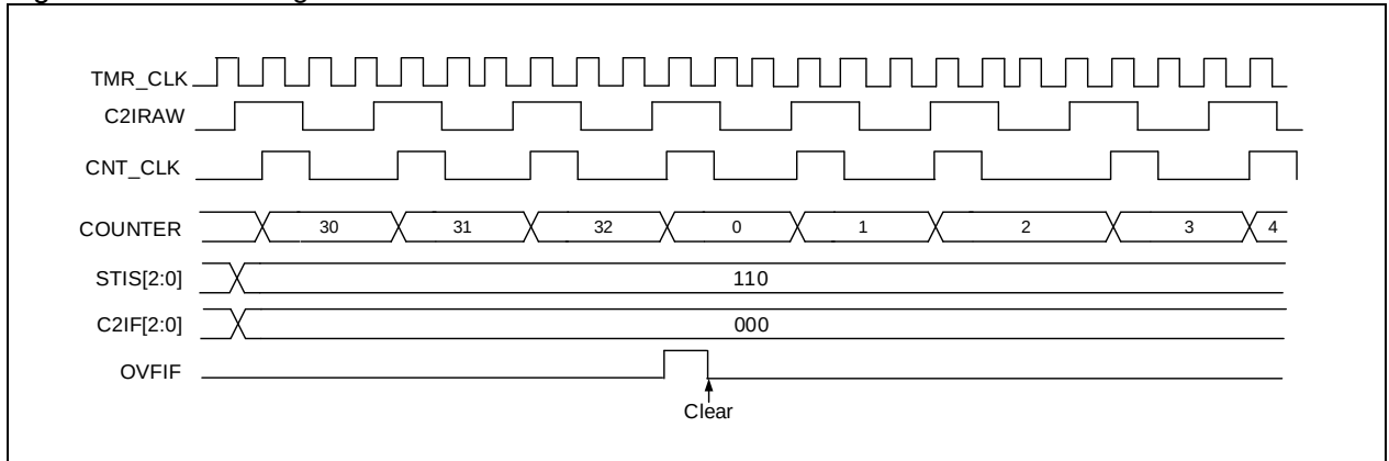
Figure 14-36 Counting in external clock mode A
