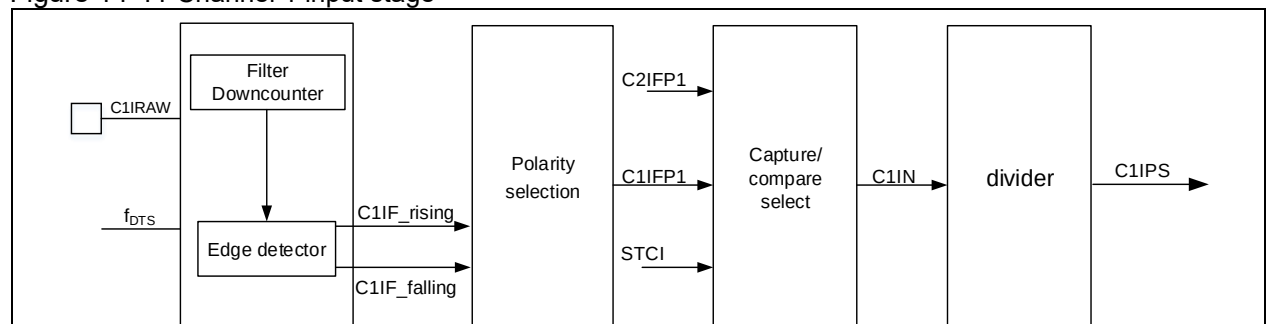
Figure 14-41 Channel 1 input stage
