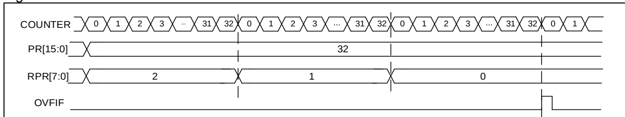
Figure 14-60 OVFI when RPR=2
