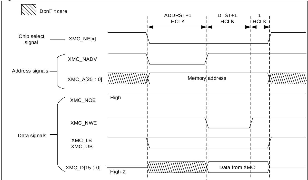
Figure 24-6 NOR/PSRAM mode 2 write access
