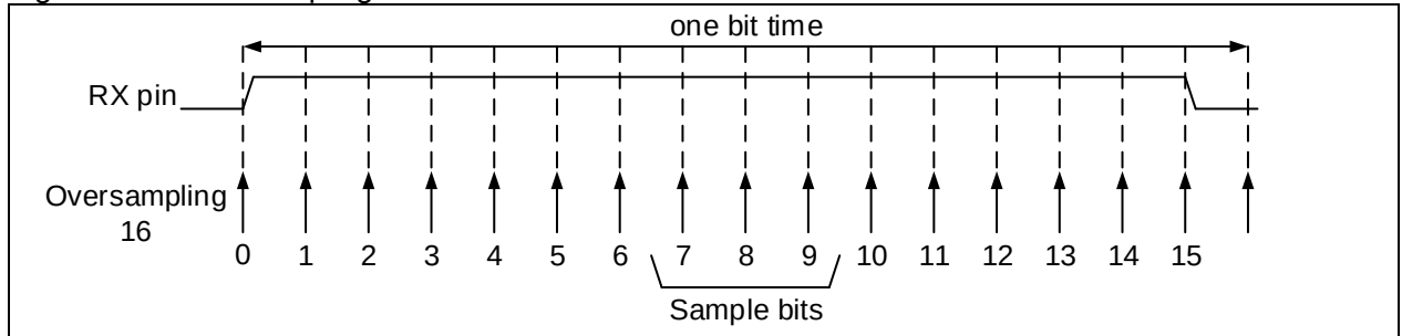
Figure 12-6 Data sampling for noise detection
