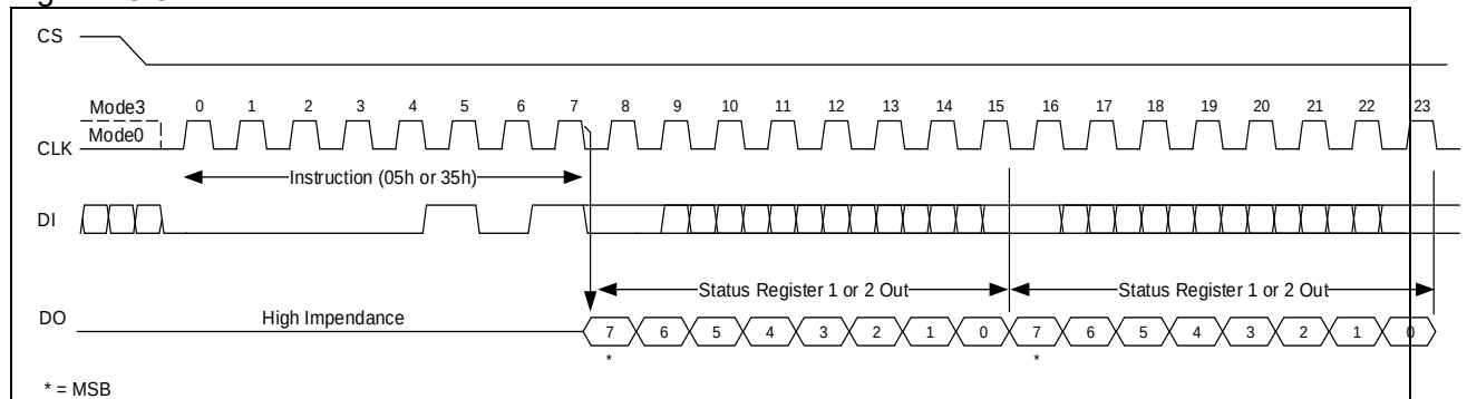
Figure 28-5 Status read
