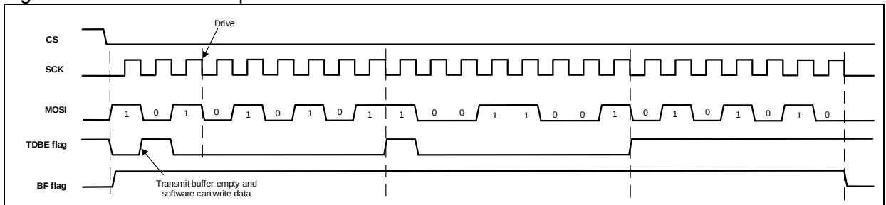
Figure 13-8 Master half-duplex transmit
