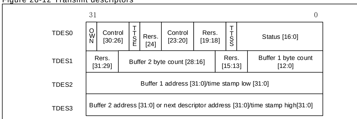
Figure 26-12 Transmit descriptors
