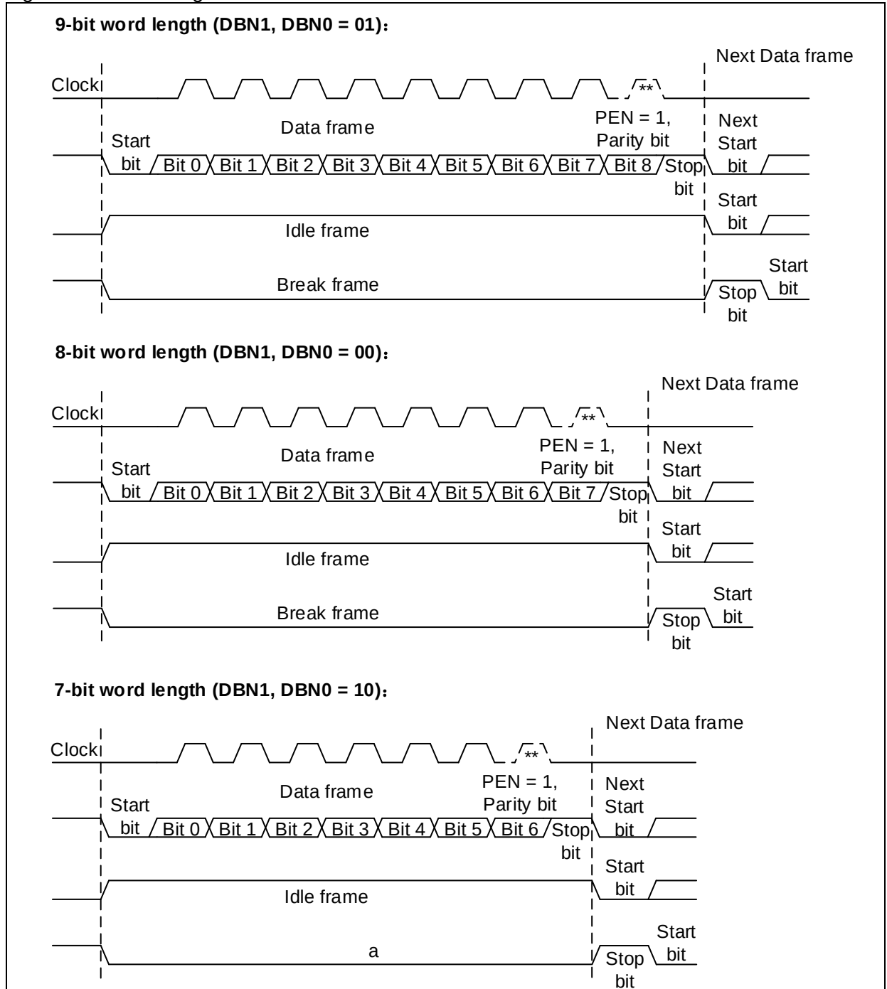
Figure 12-3 Word length
