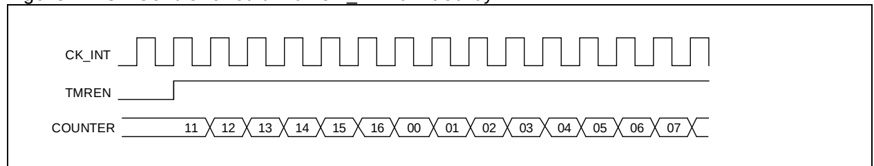
Figure 14-34 Control circuit with CK_INT divided by 1
