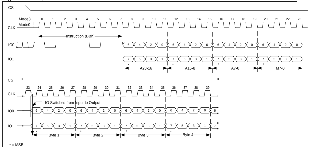
Figure 28-8 Quick read dual-wire I/O
