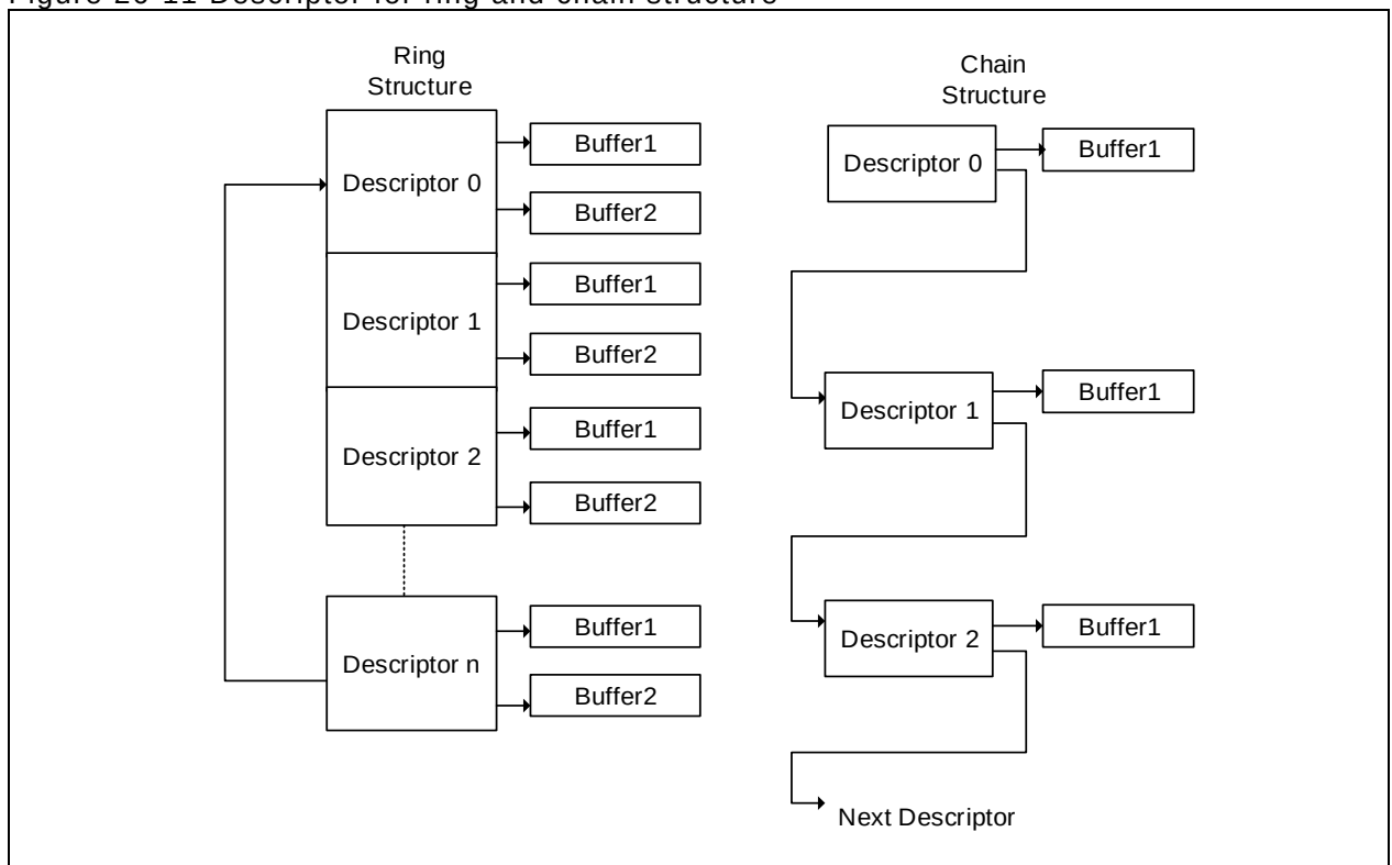
Figure 26-11 Descriptor for ring and chain structure
