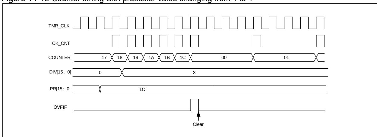
Figure 14-12 Counter timing with prescaler value changing from 1 to 4
