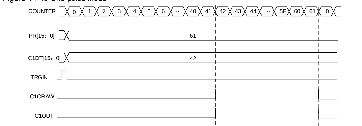
Figure 14-45 One-pulse mode
