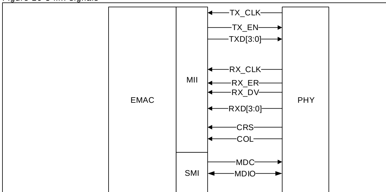
Figure 26-3 MII signals
