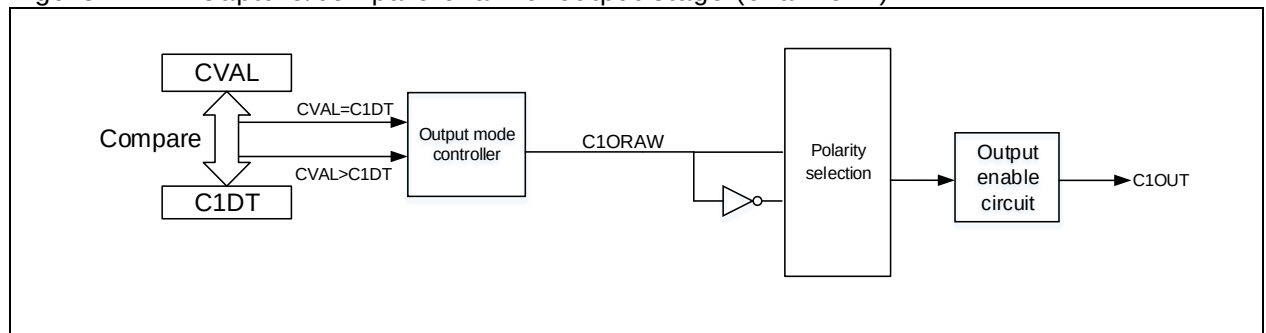
Figure 14-42 Capture/compare channel output stage (channel 1)
