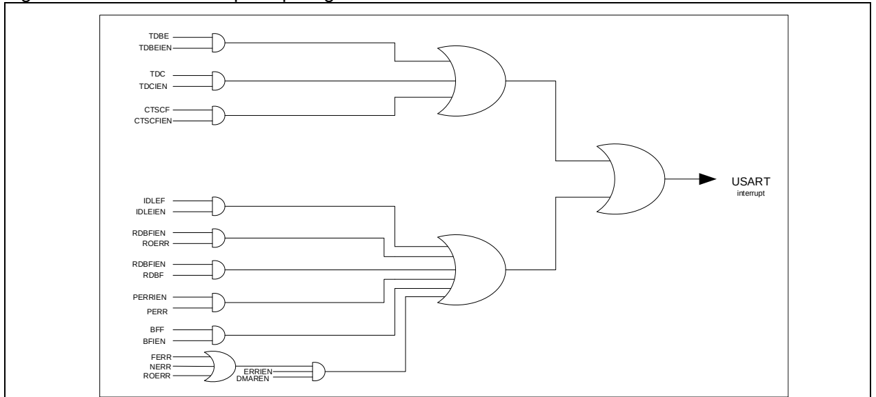
Figure 12-8 USART interrupt map diagram
