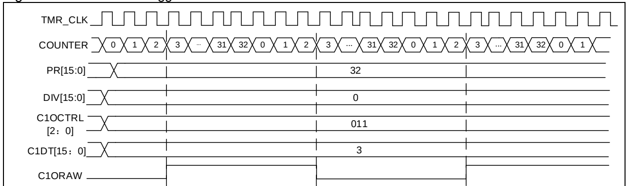
Figure 14-67 Upcounting mode and PWM mode A
