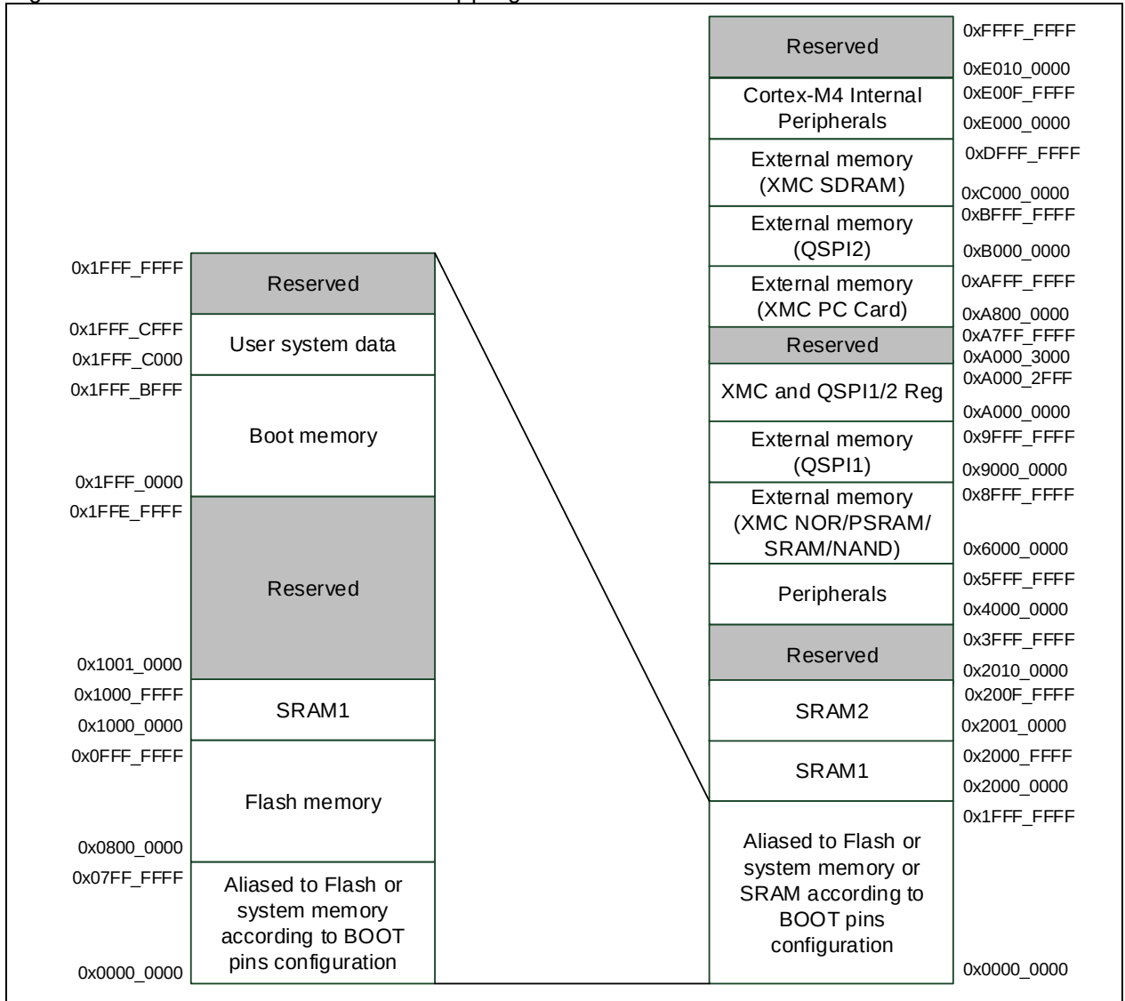
Figure 2-1AT32F435/437 address mapping
