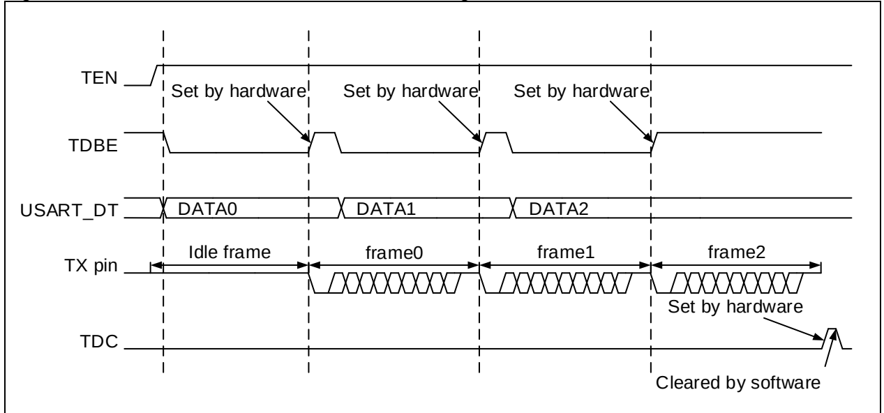
Figure 12-5 Behavior of TDC/TDBE when transmitting
