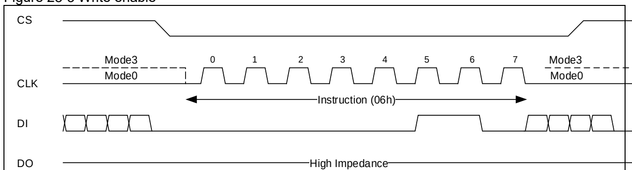
Figure 28-3 Write enable
