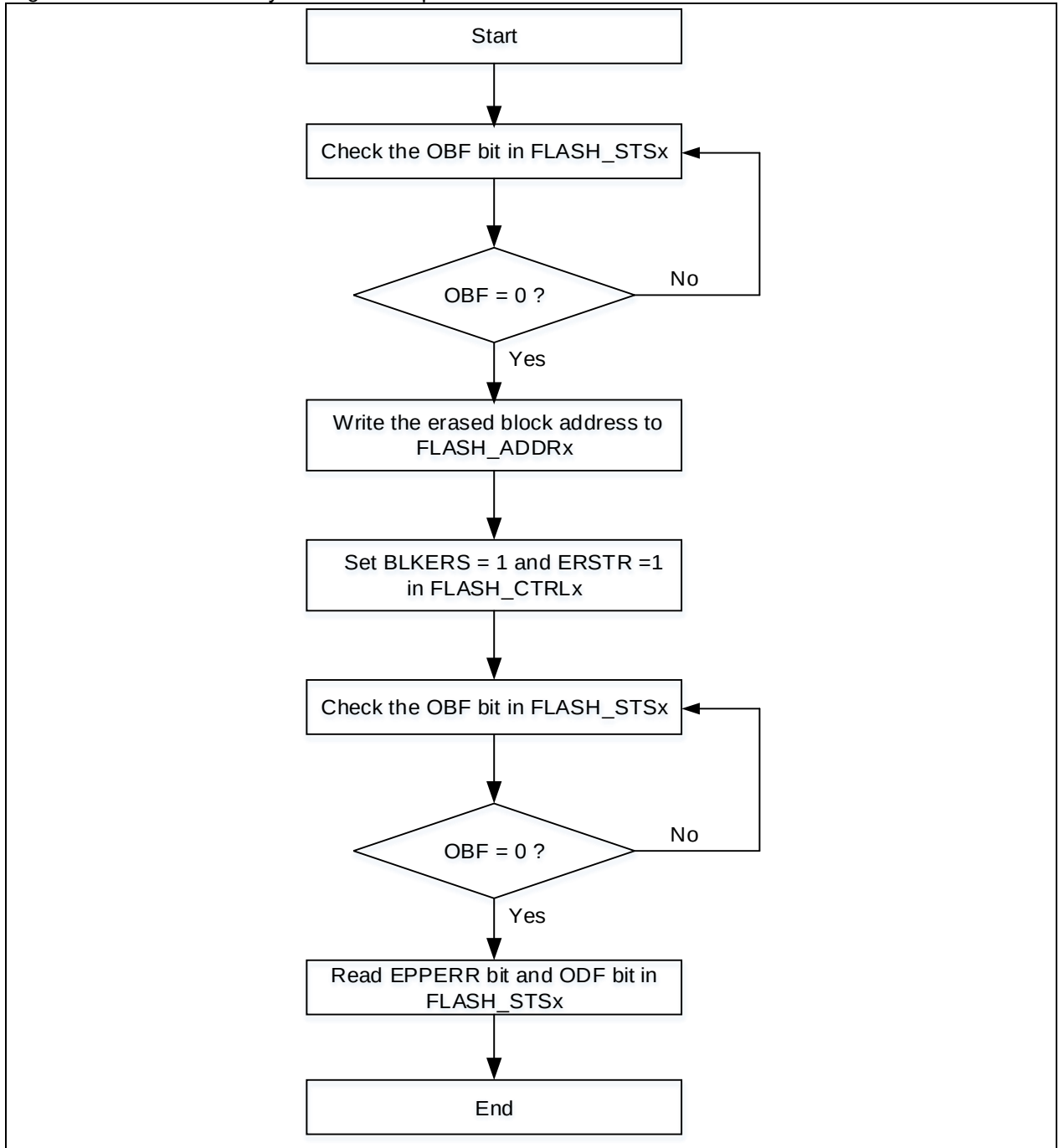
Figure 5-2 Flash memory sector erase process
