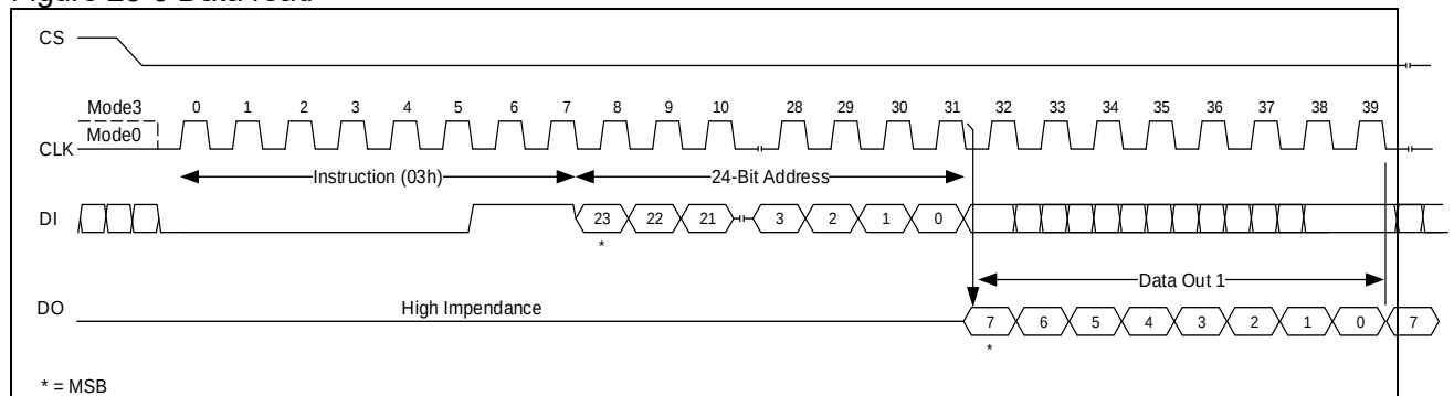
Figure 28-6 Data read
