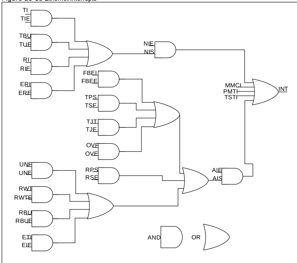
Figure 26-18 Ethernet interrupts
