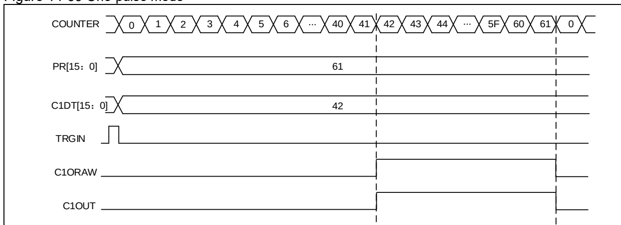
Figure 14-69 One-pulse mode
