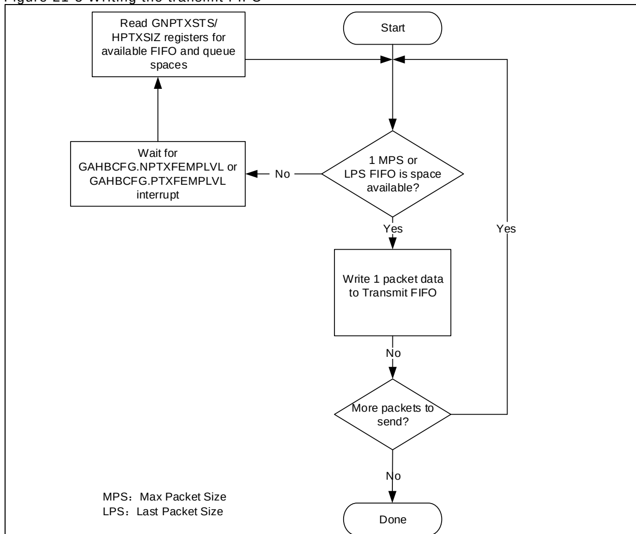
Figure 21-3 Writing the transmit FIFO
